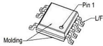
ISO View
